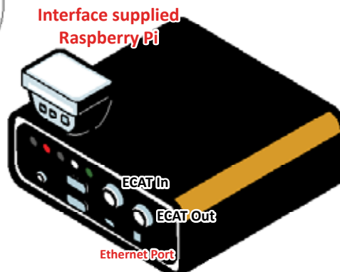
BX8-HD44 EC High Speed Data Acquisition System
