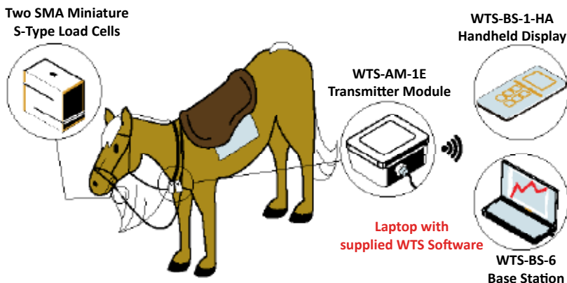
Horse with Reins
